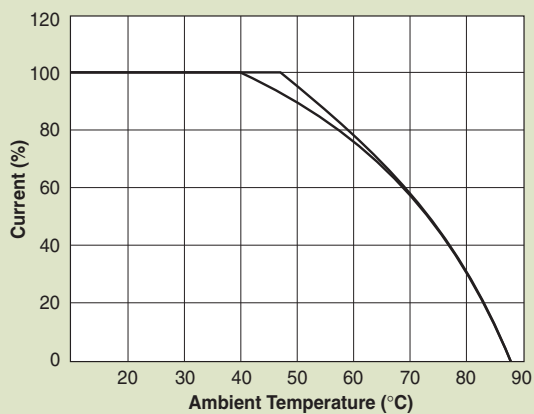
Temperature Characteristics
