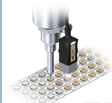
LED potting shape measurement
