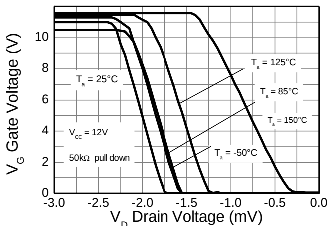
Transfer Characteristic
