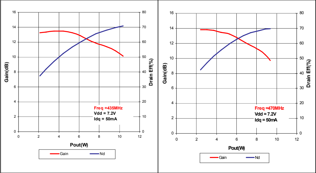
Figure 4. Gain and efficiency vs. output power Freq = 435 Mhz
