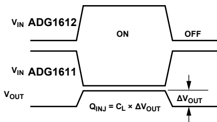
Figure 33. Charge Injection
