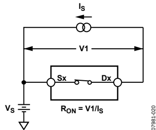
Figure 24. On Resistance
