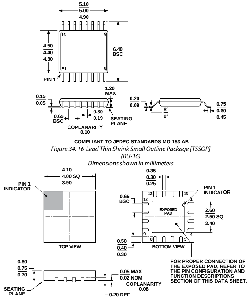
COMPLIANT TO JEDEC STANDARDS MO-220-WGGC. Figure 35. 16-Lead Lead Frame Chip Scale Package [LF CSP_WQ] 4 mm x 4 mm Body, Very Very Thin Quad (CP-16-26) Dimensions shown in millimeters
