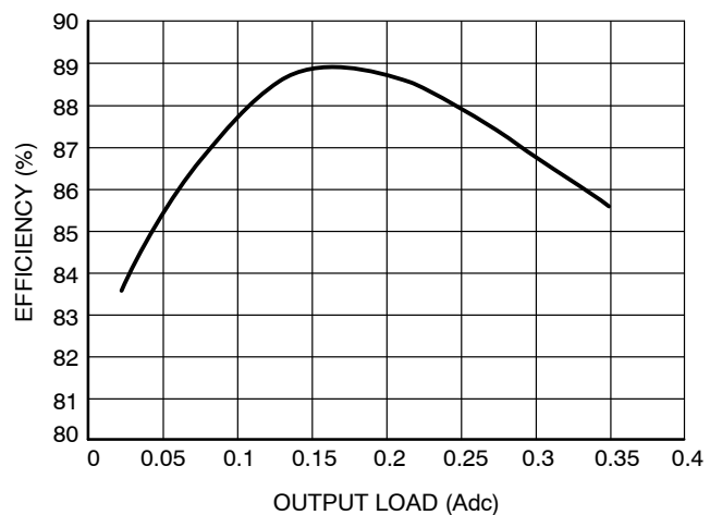
Figure 21. Efficiency vs. Output Current for the Boost Demo Board at V_{in} = 12\text{ V} , V_{out} = 24\text{ V} , T_A = 25^\circ\text{C}
