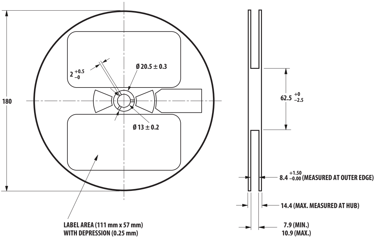
Figure 12: Reel Dimensions
