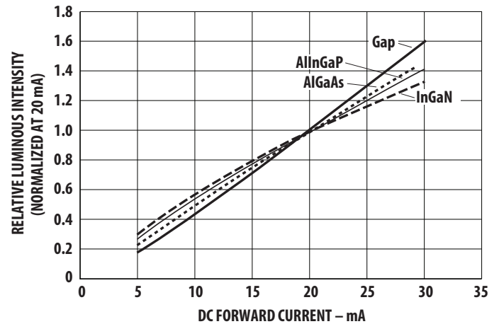
Figure 3: Relative Intensity vs. Forward Current
