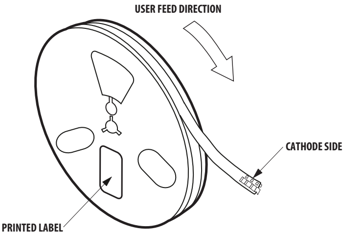
Figure 13: Reeling Orientation
