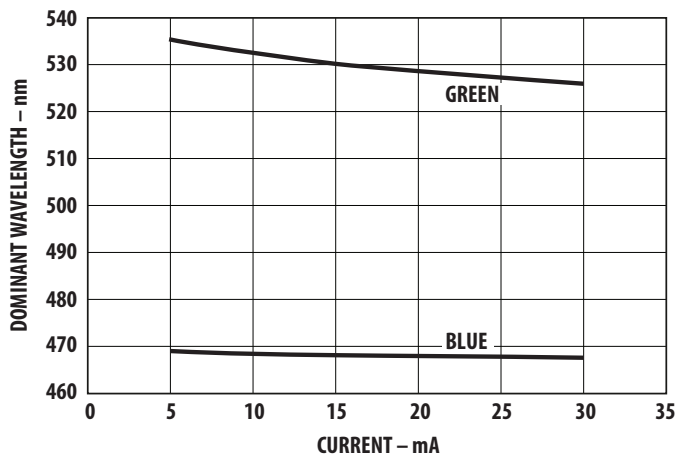
Figure 6: Dominant Wavelength vs. Forward Current (InGaP Devices)
