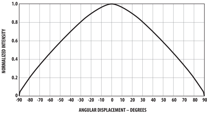
Figure 8: Radiation Pattern
