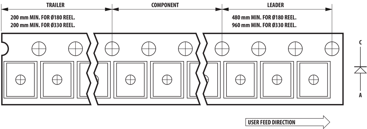
Figure 11: Tape Dimensions
