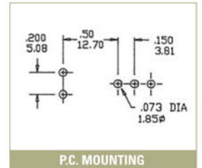
P.C. MOUNTING
