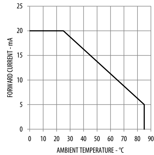
Figure 10: Derating Curve
