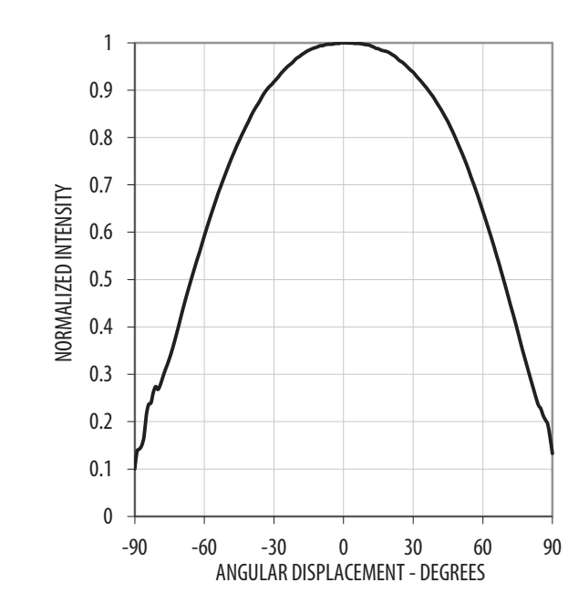
Figure 5: Radiation Pattern
