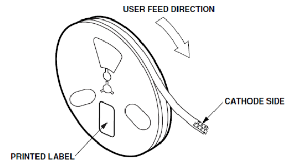
Figure 12: Reel Orientation
