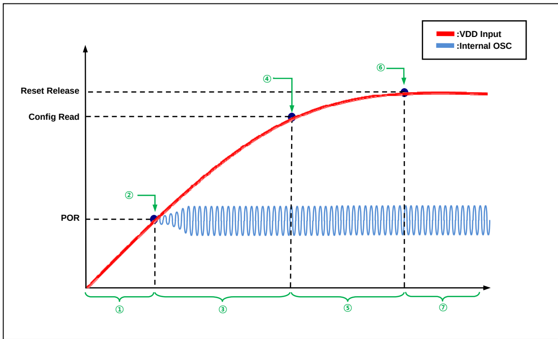
Figure 13-6 Boot Process Waveform
