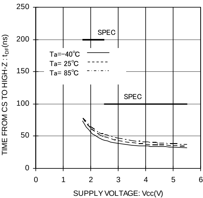
Figure 32. Time from CS to High-Z vs Supply Voltage
