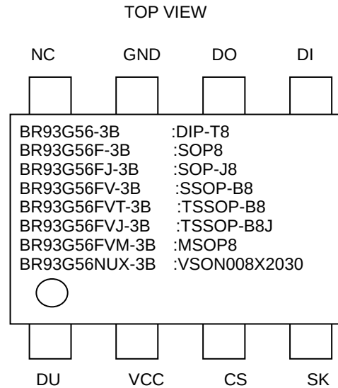
Figure 3. Pin Configuration
