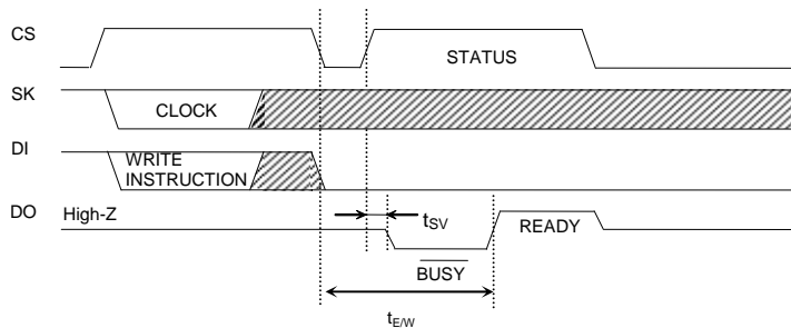
Figure 48. \overline{READY} / \overline{BUSY} STATUS Output Timing Chart
