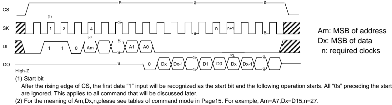
Figure 35. Read Cycle
