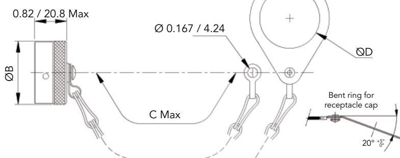
Cap for receptacle Type 502
