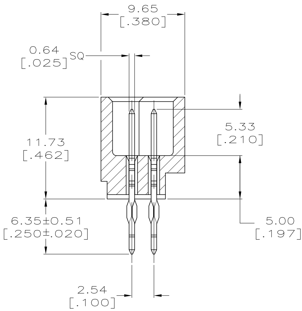
SECTION T-T
