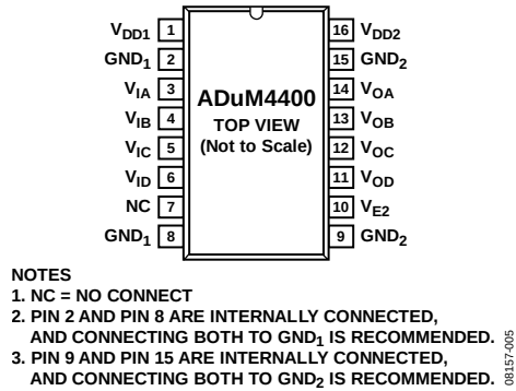
Figure 5. ADuM4400 Pin Configuration
