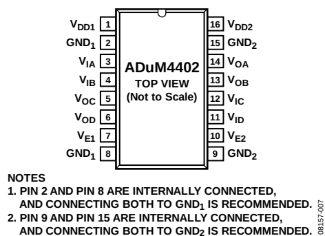
Figure 7. ADuM4402 Pin Configuration
