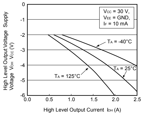
HIGH LEVEL OUTPUT VOLTAGE vs. HIGH LEVEL OUTPUT CURRENT
