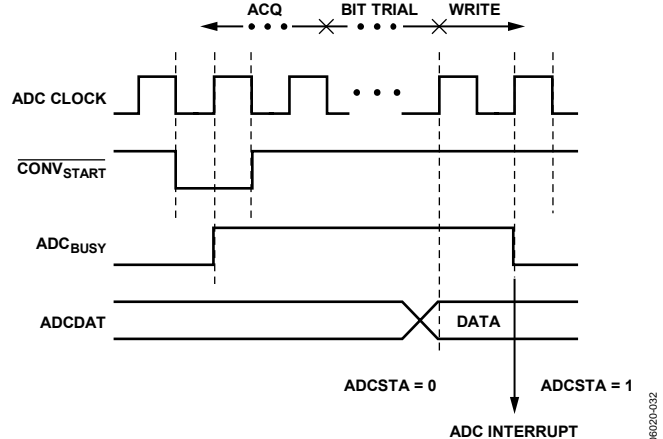
Figure 36. ADC Timing
