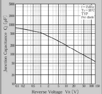
Junction Capacitance
