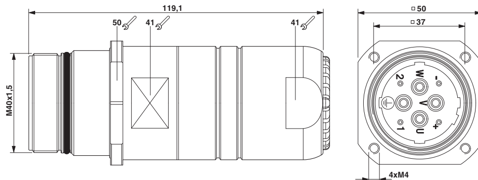
Dimensioned drawing
