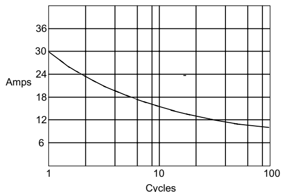
Figure 2 Maximum Forward Surge Current
