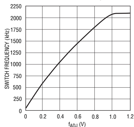
Switch Frequency vs f_{\text{ADJ}}
