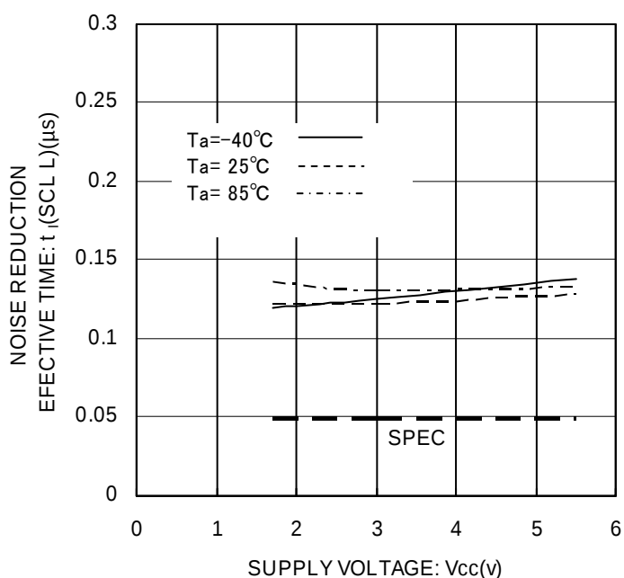
Figure 29. Noise Spike Width t_I (SCL L)
