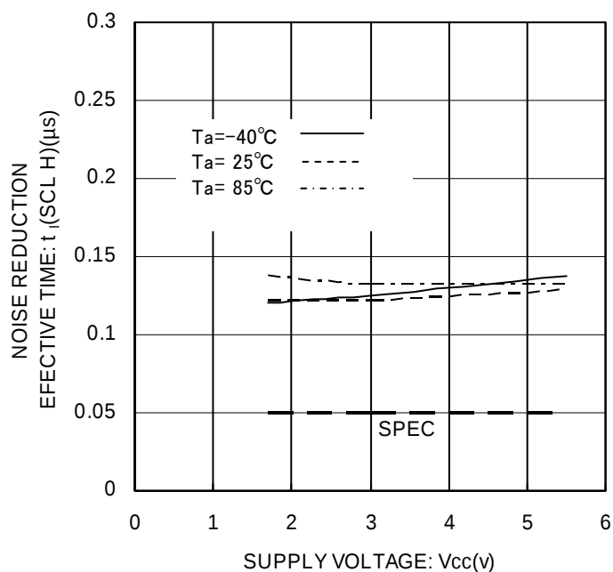
Figure 28. Noise Spike Width t_I (SCL H)
