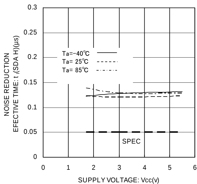
Figure 30. Noise Spike Width t_I (SDA H)
