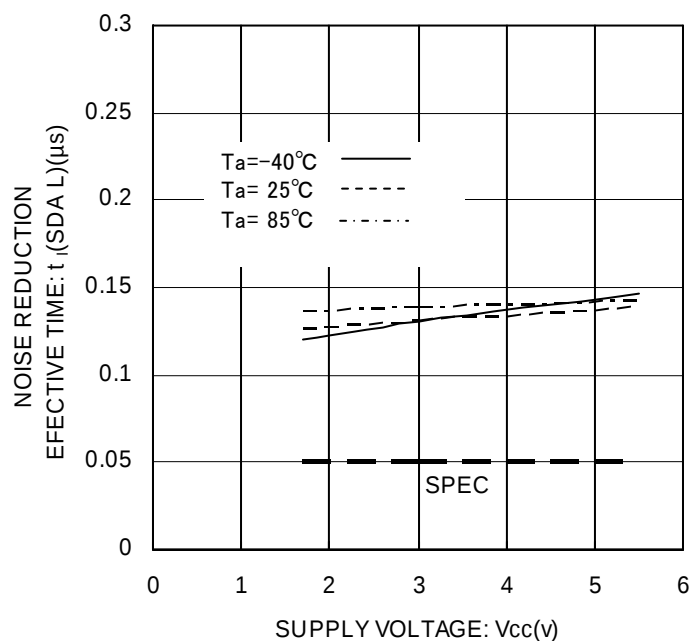
Figure 31. Noise Spike Width t_I (SDA L)
