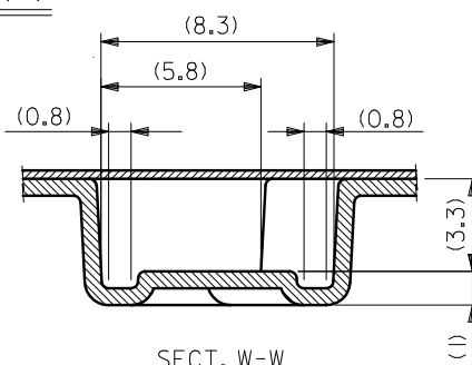
SECT. W-W
