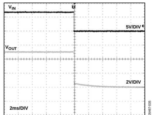
Figure 31. ADR361 Turn-Off Response Time, 0.1 \mu F Output Capacitor
