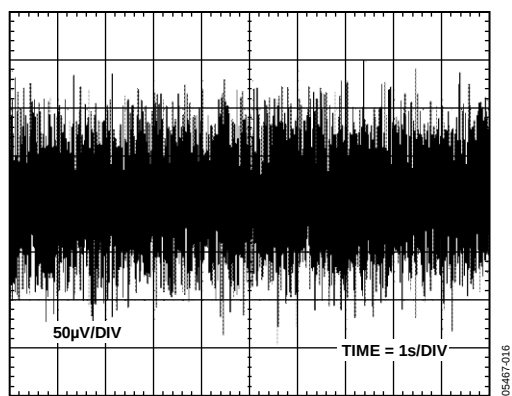
Figure 18. ADR363 10 Hz to 10 kHz Noise
