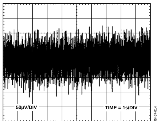
Figure 16. ADR361 10 Hz to 10 kHz Noise
