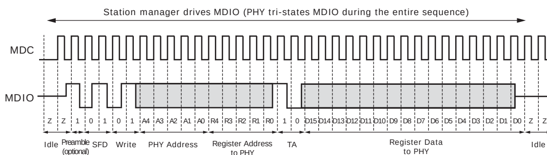
Figure 14 • SMI Write Frame
