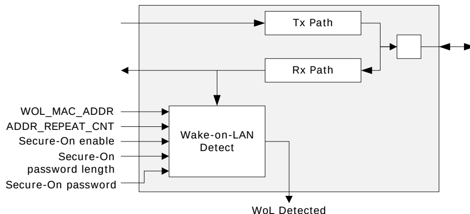
Figure 16 • Wake-on-LAN Functionality
