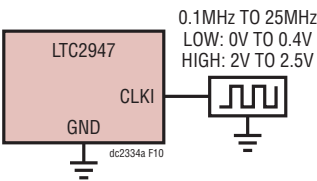
Figure 10. LTC2947 in External Clock Operation
