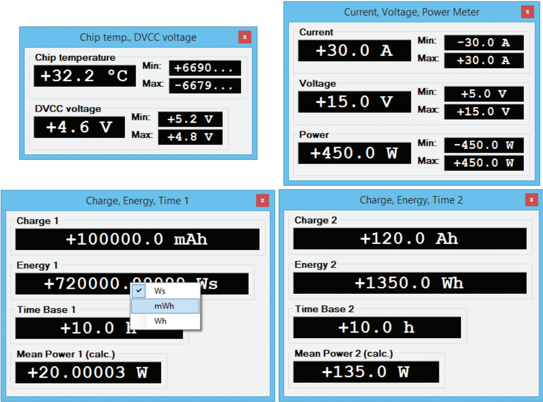
Figure 20. GUI Multimeters for All Measurement Quantities
