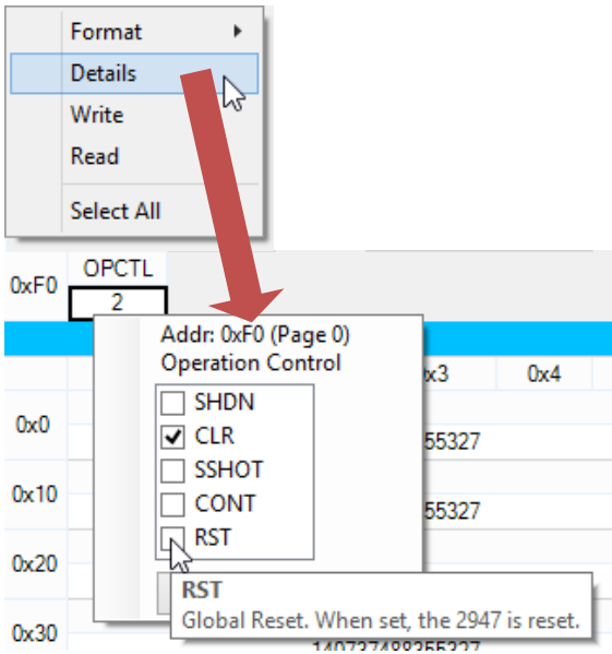
Figure 49. Register Details View
