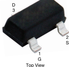
SOT-23 (TO-236)
