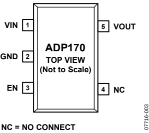
Figure 3. ADP170 5-Lead TSOT
