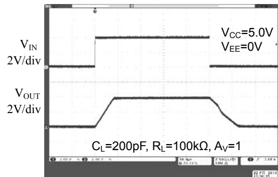
Time (10μs/div)
