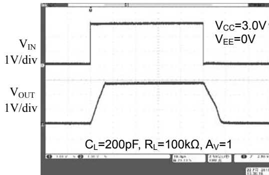
Time (10μs/div)
