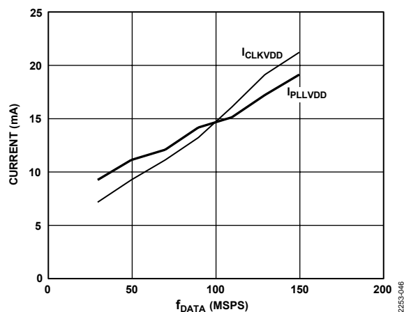
Figure 46. I_{PLLVDD} and I_{CLKVDD} vs. f_{DATA}
