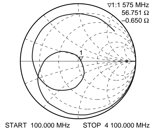
S 22 —FREQUENCY
