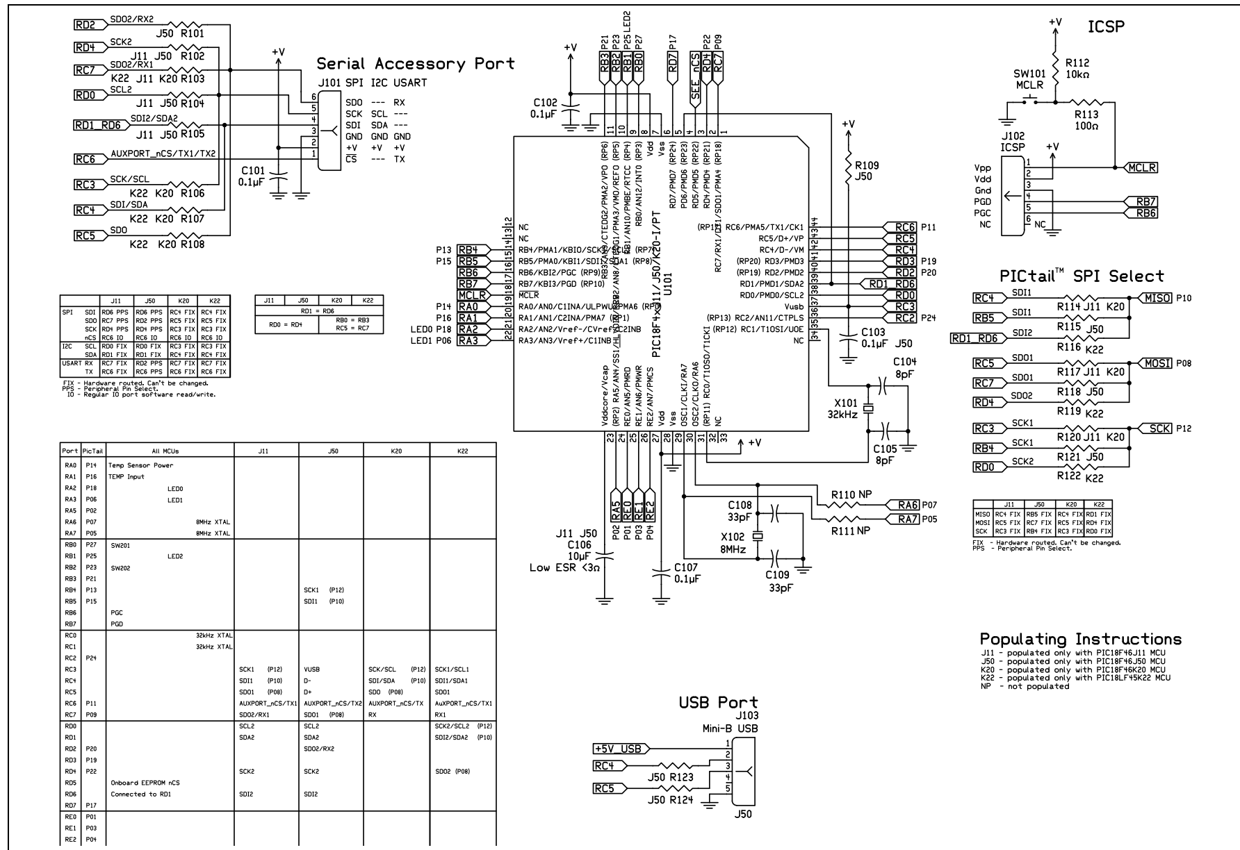
FIGURE A-1: PIC18 WIRELESS DEVELOPMENT BOARD SCHEMATIC
