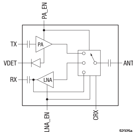
Figure 1. SKY85703-11 Block Diagram
