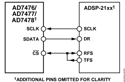
Figure 27. Interfacing to the ADSP-21xx
