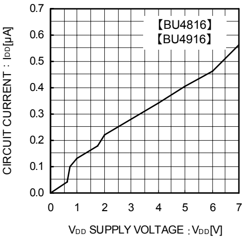
Fig.3 Circuit Current
