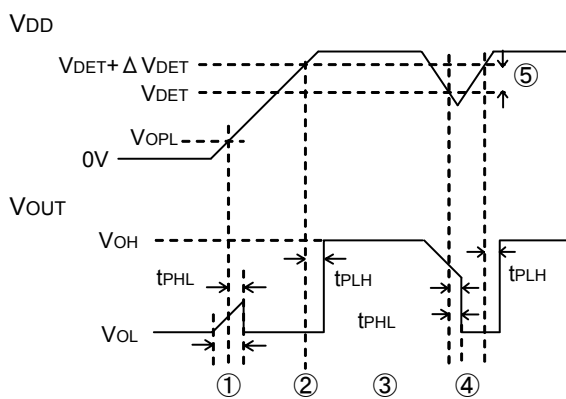
Fig. 14 Timing Waveforms
