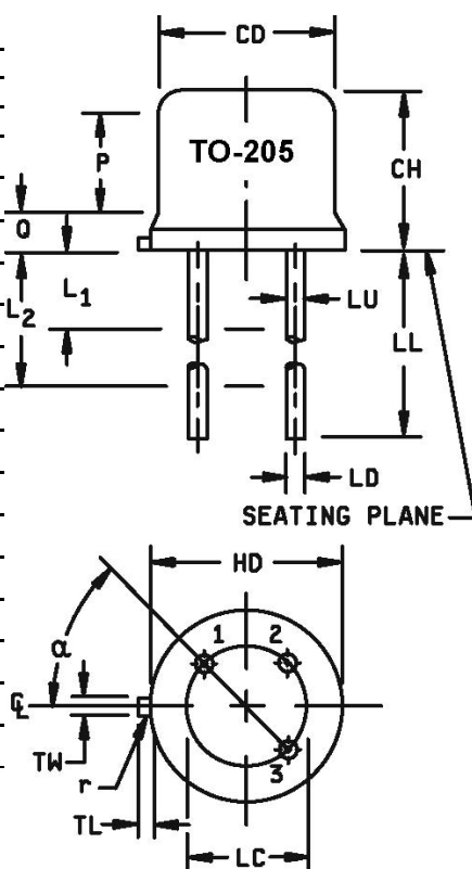
FIGURE 1 (TO-5, TO-39) PACKAGE DIMENSIONS
