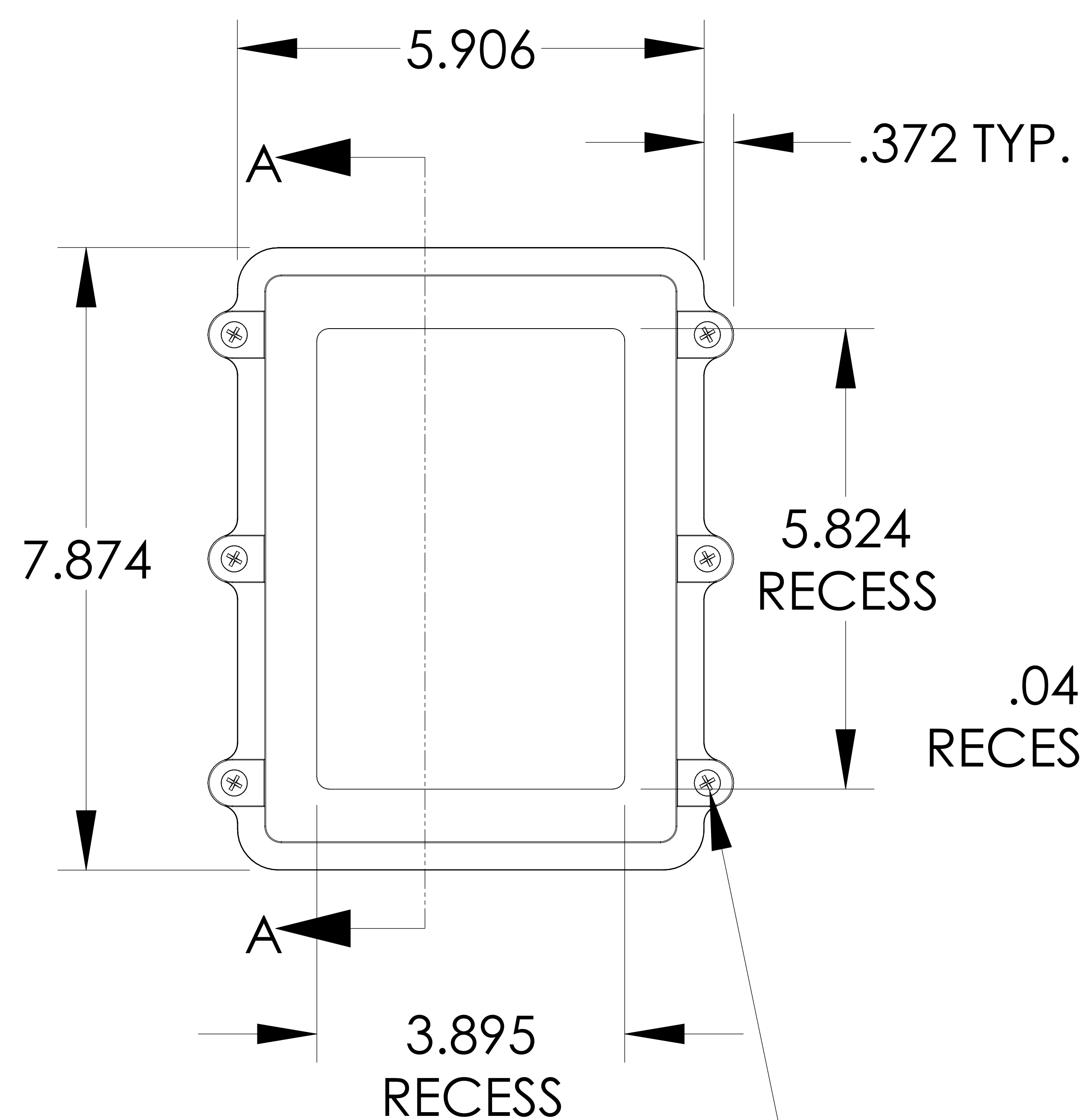
TOP VIEW
