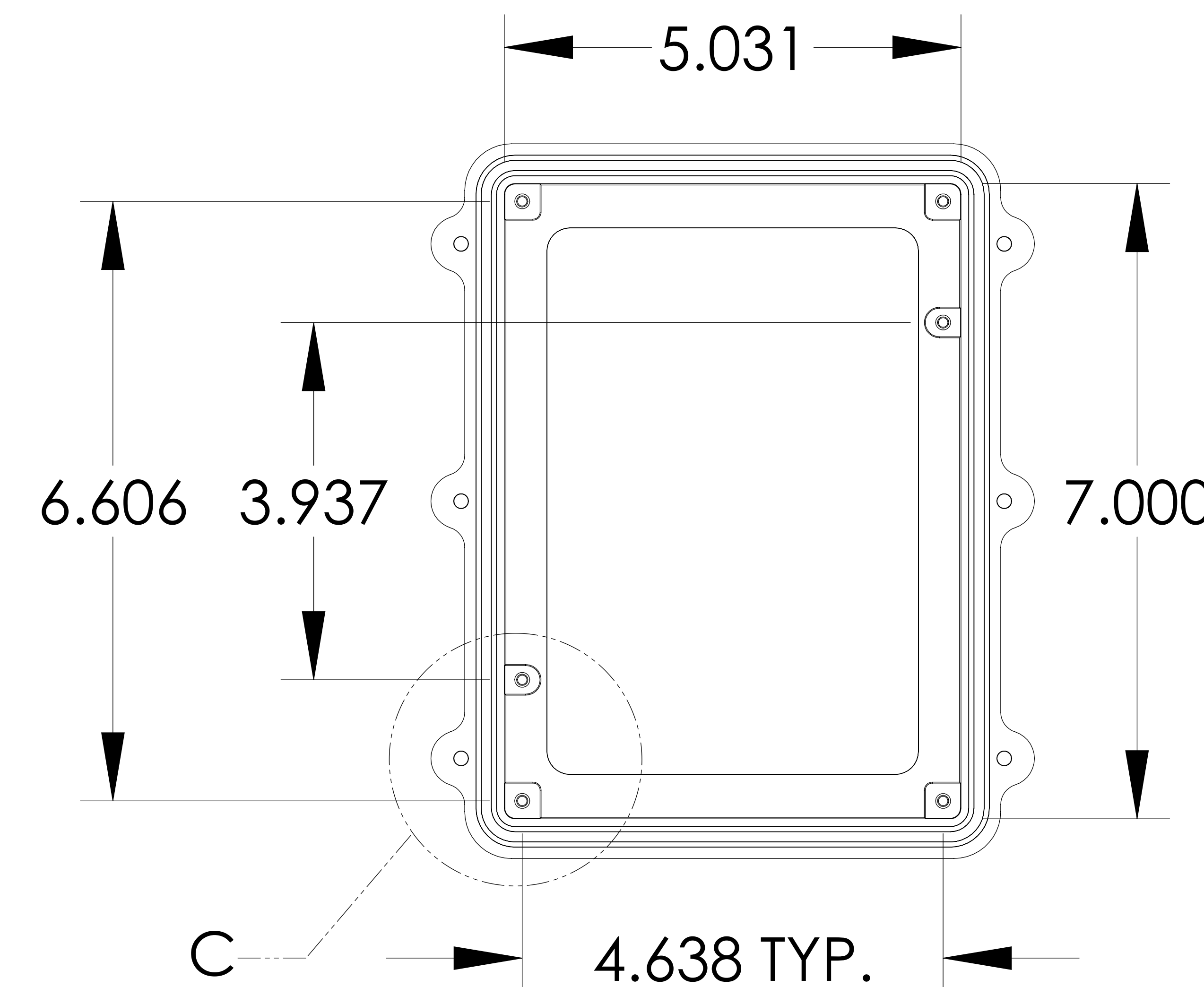
INSIDE COVER DETAILS
