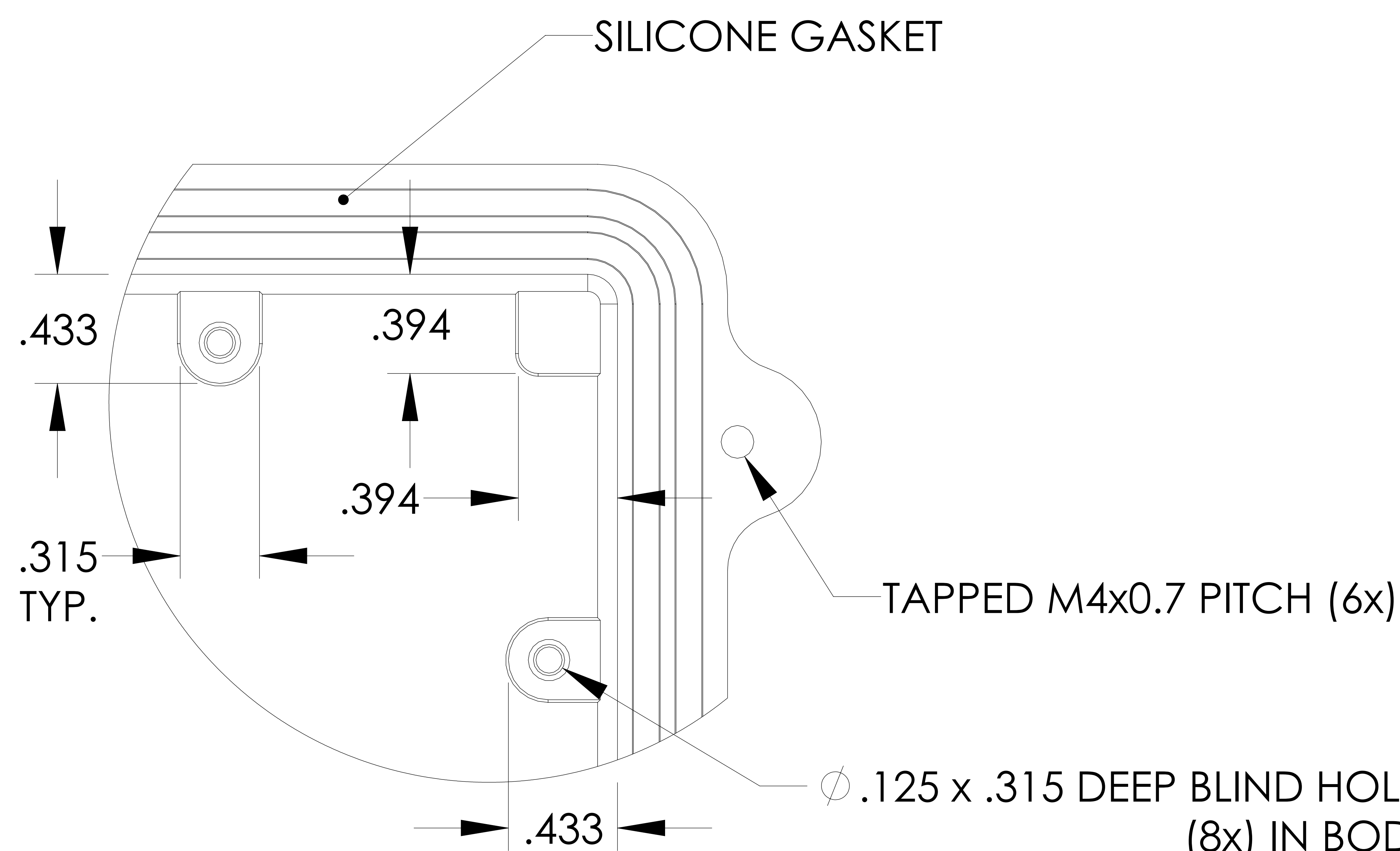
DETAIL B SCALE 4 : 1
