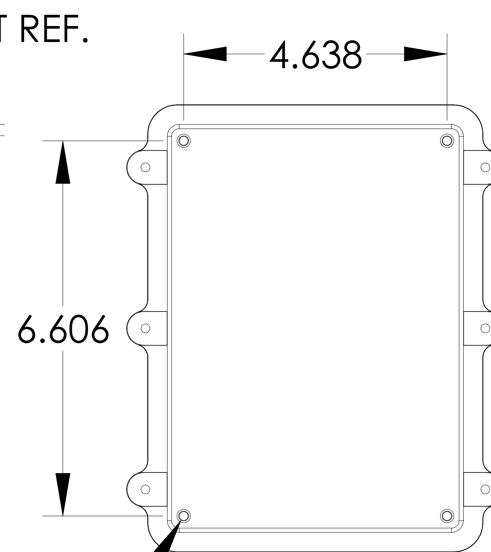
BOTTOM VIEW
