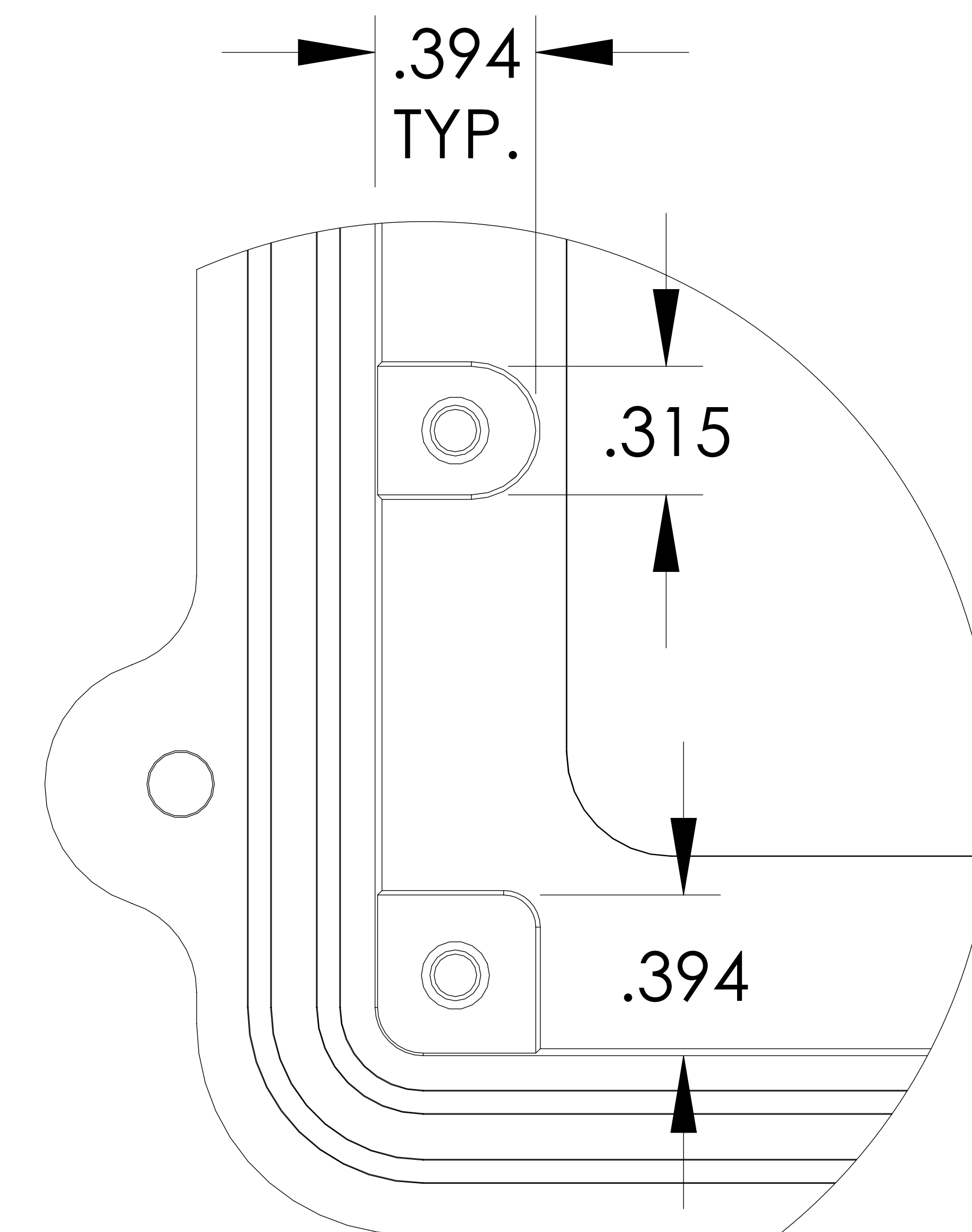
DETAIL C SCALE 4 : 1
