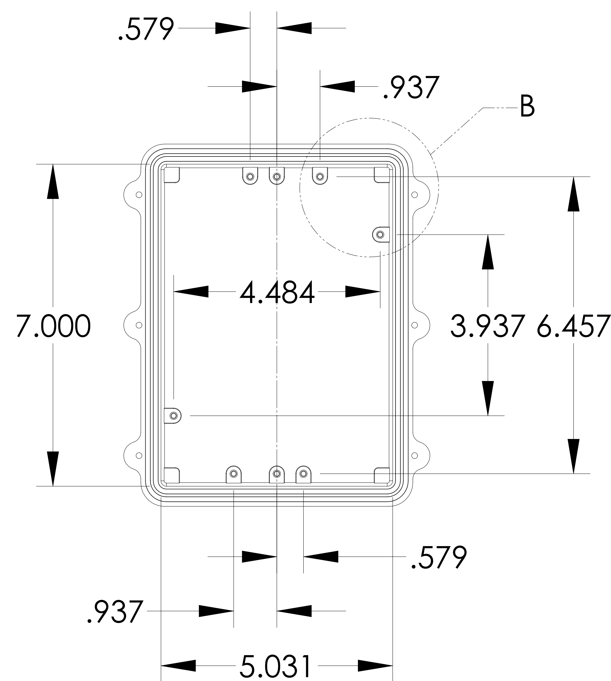
INSIDE BODY DETAILS
