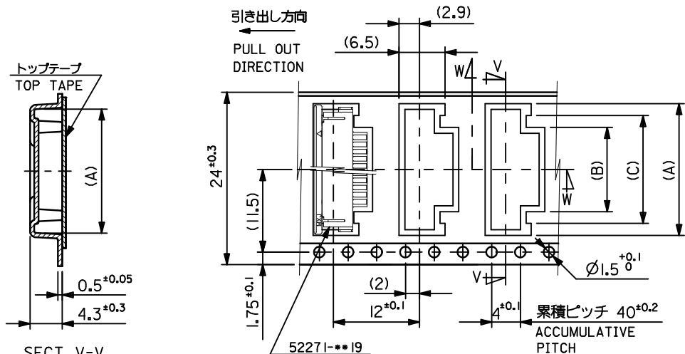
SECT. V-V
