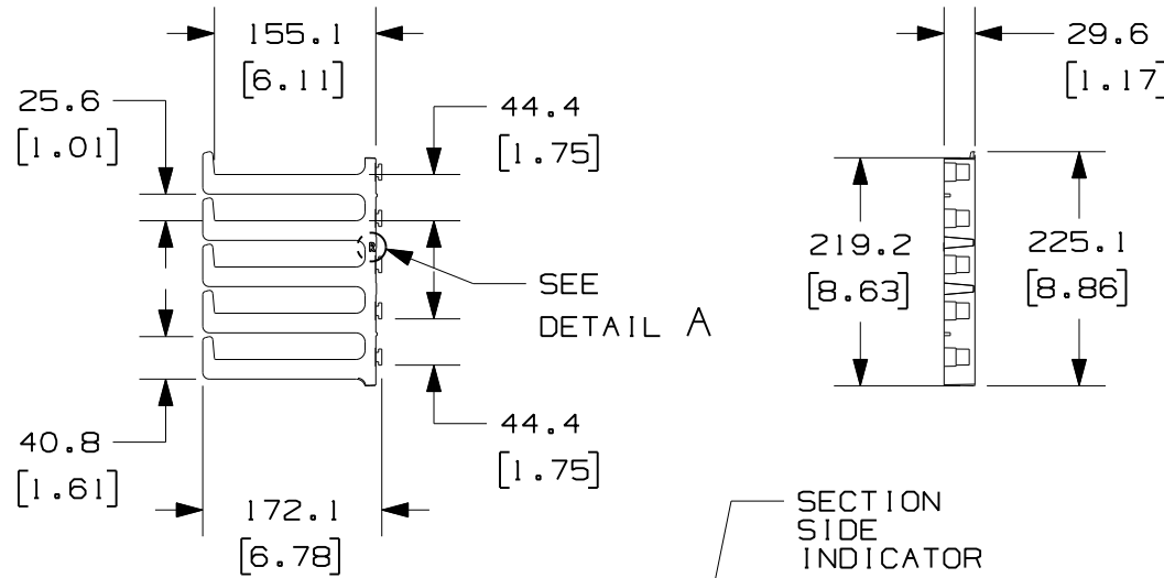
5RU CABINET FINGER SECTION-RIGHT HAND
