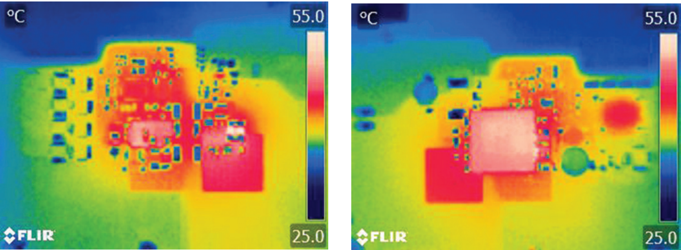
Figure 1. Thermal Pictures – V_{PORT} = 57V, 24V/0.95A
