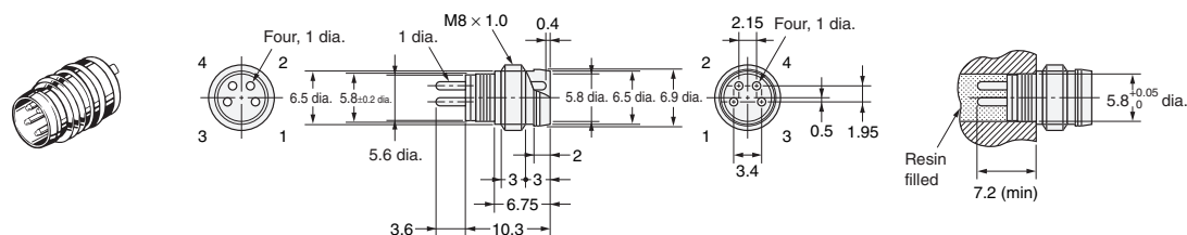
Mounting Dimensions
