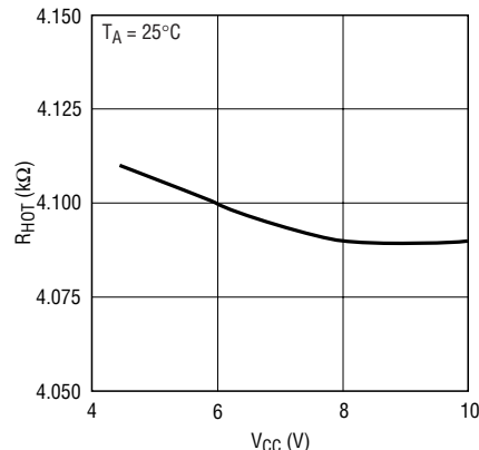
NTC R_{HOT} Threshold Voltage vs V_{CC}
